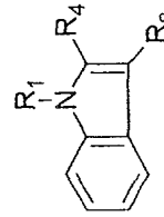
Ligand E IC_{50} = 3.2 \times 10^{-6} M
